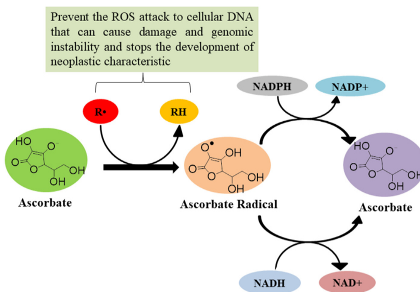
Figure 9. Antioxidant mechanism of ascorbic acid [40,41,71].
