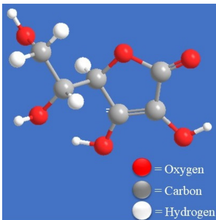
Figure 1. Chemical structure of ascorbic acid.
