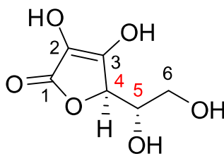
Figure 4. Numbering of the different carbon atom of L-ascorbic acid (4R, 5S).
