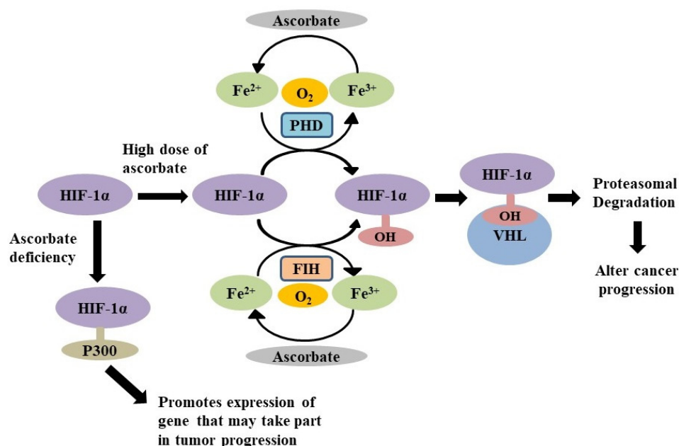
Figure 6. Ascorbate regulates HIF-1 \alpha by recycling Fe 2+ required for the function of PHDs and FIH, leading to alteration of cancer progression [34,35,37,41,42].
