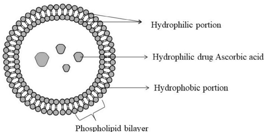
Figure 12. Structure of liposome.
