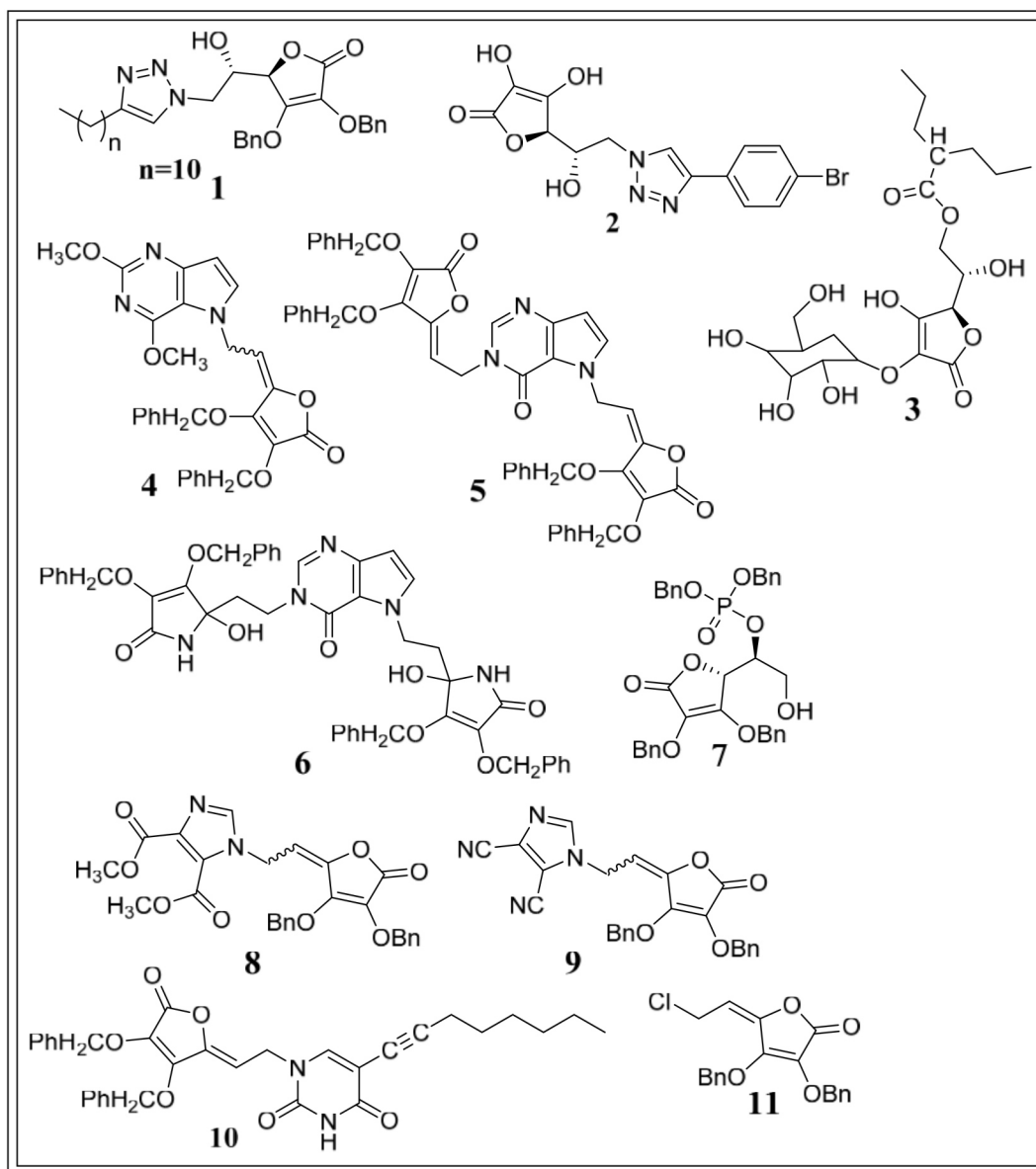
Figure 10. Ascorbic acid analogues showing antitumor effects.
