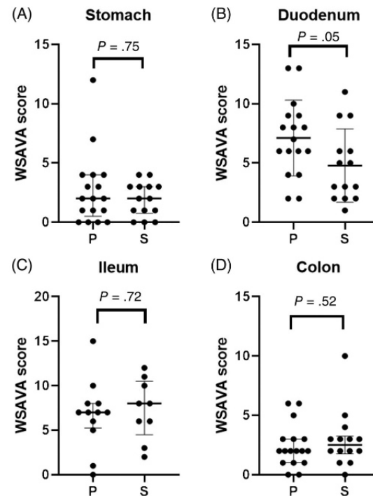
FIGURE 2 World Small Animal Veterinary Association (WSAVA) histology scores 14 (A, stomach; B, duodenum; C, ileum; and D, colon) from 31 dogs with protein-losing enteropathy (PLE) treated with prednisolone alone (group P) or with prednisolone and a second-line immunosuppressant (group S). A and D present data as median (horizontal bar) and interquartile range (whiskers). B and C present data as mean (horizontal bar) and SD (whiskers)
